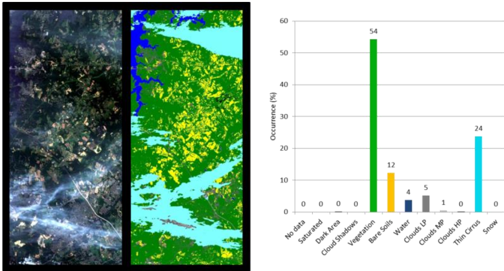
Figure 2-6 – Scene Classification
