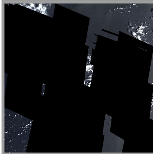
Figure 2-14 – L2A TCI image of a tile processed with a Quality Mask masking defective pixels of different affected bands.
